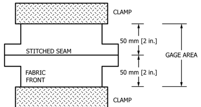
FIG. 2 (a) Placement of Generic Seam in Clamps for Sewn Seam (Front View)
