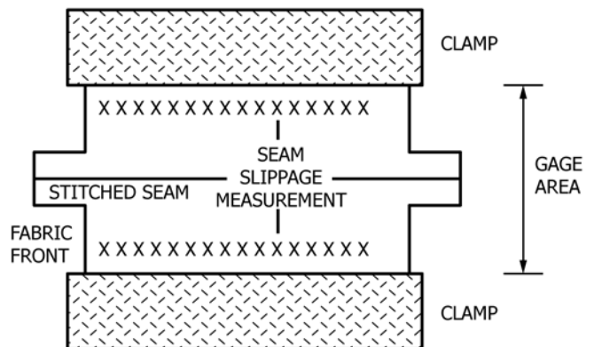
FIG. 3 (a) Gage Area for Measurement of Geotextile/Seam Slippage of Sewn Seam Specimen
