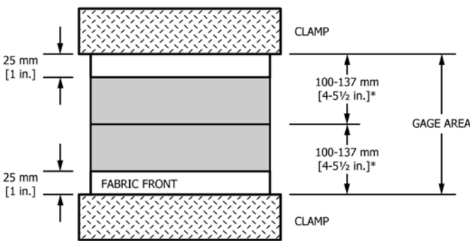
FIG. 2 (c) Placement of Generic Seam in Clamps for Adhesive Bonded Seam (Front View) (continued)
